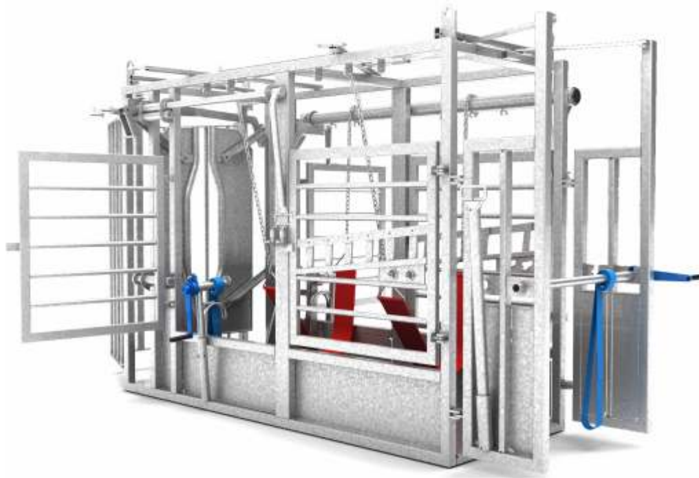
View of veterinary chute with additional equipment.
